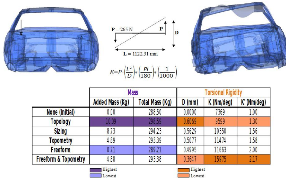
Figure 8: Results of Stiffness Optimization using Different Structural Optimization Types
