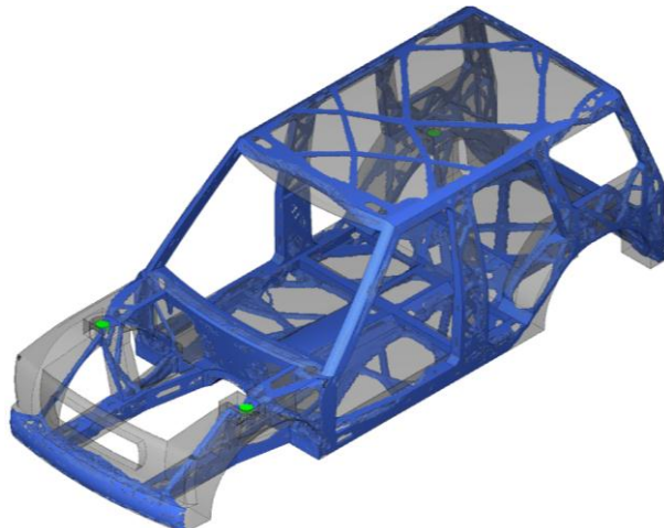
Figure 2: Topology Optimization of Vehicle
