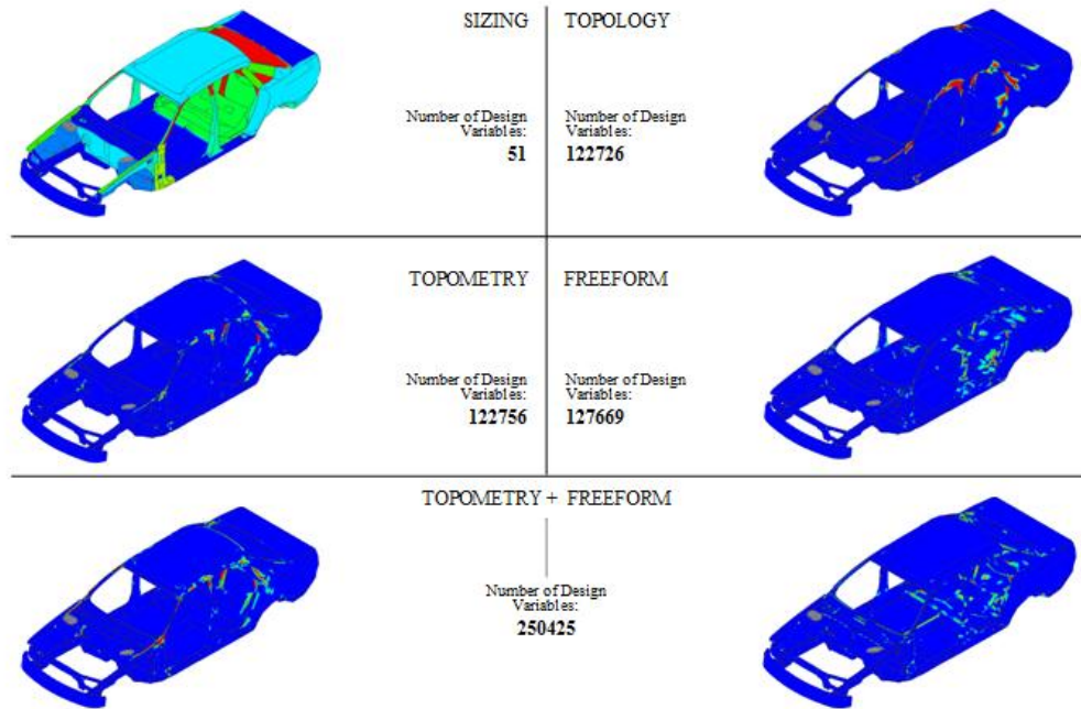
Figure 10: Results of Stiffness Optimization using Different Structural Optimization Types
