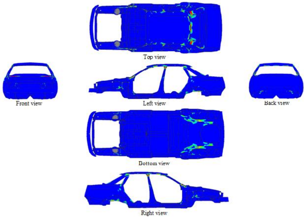
Figure 5: Optimal Places to Reinforce a Car Body using Topometry Optimization
