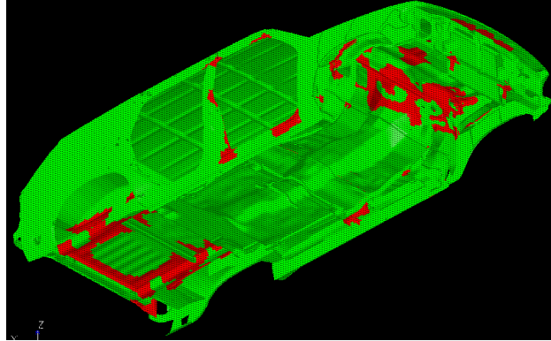
Figure 3: Topology Optimization of Vehicle. Red Areas Show Optimal Areas to Reinforce
