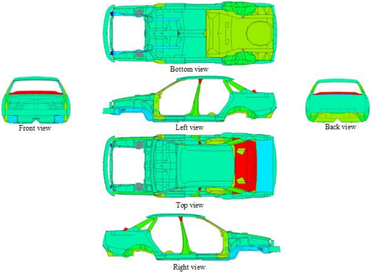
Figure 4: Thickness Distribution using Sizing Optimization
