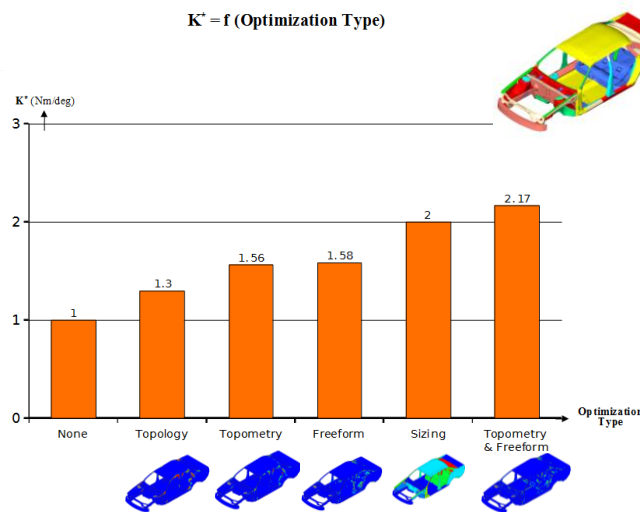
Figure 9: Results of Stiffness Optimization using Different Structural Optimization Types
